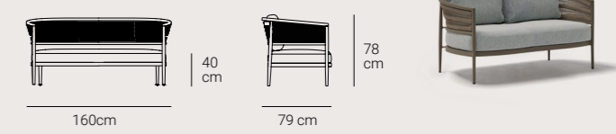
LOVE SEAT SL53201
